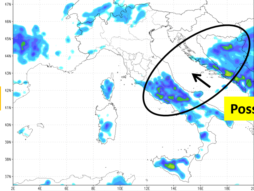
Total Precipitation [mm/3h] 0.4 0.6 1 3 5 7 10 15 25 30 40 60 70 80 100 125 150 175 200 250 300 350
